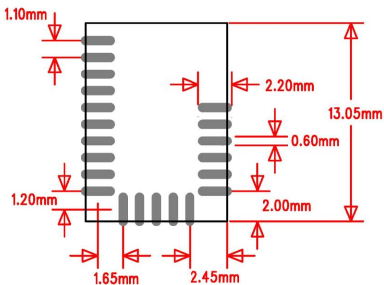
Figure 4: Recommended PCB land pattern
